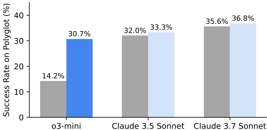
Model Transfer on Polyglot
