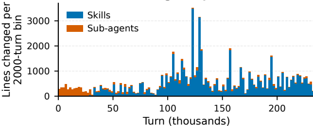
(a) Skill and sub-agent updates
