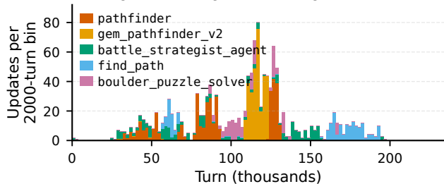
(b) Top-5 most-updated components
